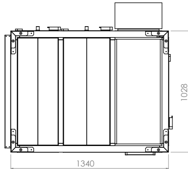
Taban-Base Plan
