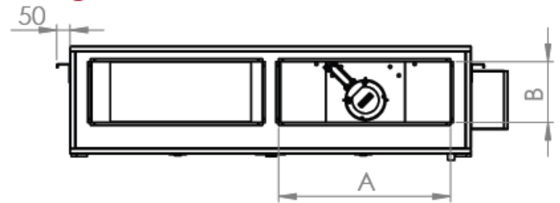
Right View
